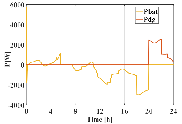
Fig. 12. Evolution of daily energy management
