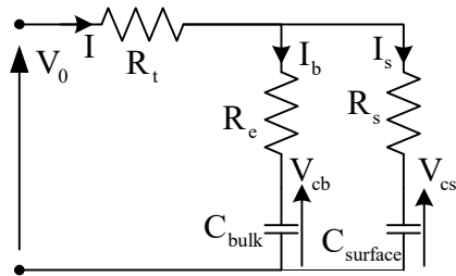
Fig. 3. Battery model diagram
