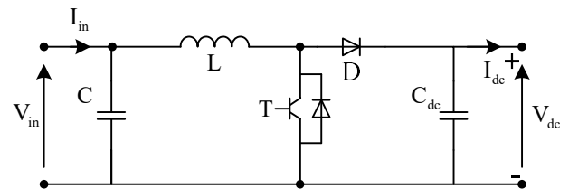
Fig. 4. The model of boost converter.
